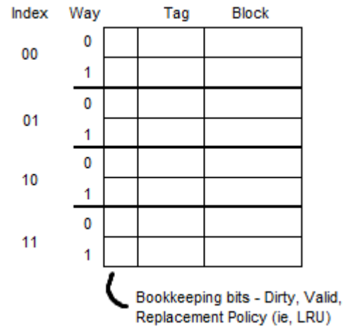
Figure 2: An 8 block, 2 way set associative cache (4 sets)
