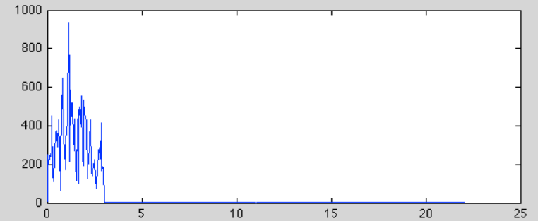
LP-Filter Spectrum
