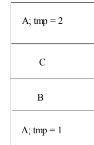
Execution stack
