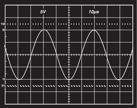
TPC 27. 20 V p-p, 25 kHz Sine Wave Input; Unity Gain Follower; R_L = 600 \Omega, V_S = \pm 15 V
