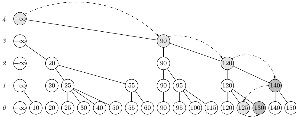
Figure 9.18: An abstract view of a skip list, showing its relationship to a (non-binary) search tree. Each key other than -\infty is duplicated to a random height. We can search this structure beginning at any level. In the best case, to search (unsuccessfully) for the target value 127, we need only look at the keys in the shaded nodes. Darker shaded nodes indicate keys larger than 127 that bound the search.
