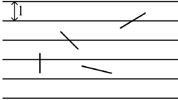
Figure 1: Buffon's Needle.
