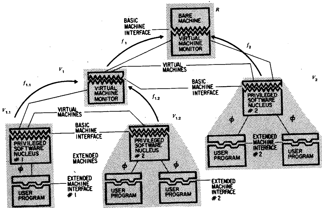
Figure 3. Virtual Machine Model with Recursion
