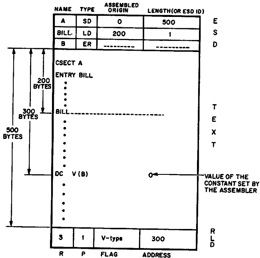
Fig. 7. Object Module One.
