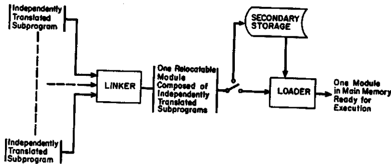
FIG. 2. Linking after translation but before loading.
