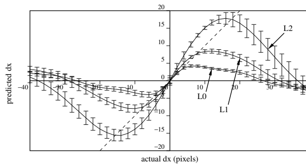
Fig. 9. Predicted dx vs actual dx for 3 levels of a Multi-Resolution model. L0: 10000 pixels, L1: 2500 pixels, L2: 600 pixels. Errorbars are 1 standard error
