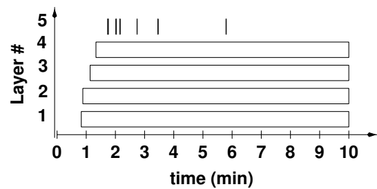
Figure 8: Simple sample path.
