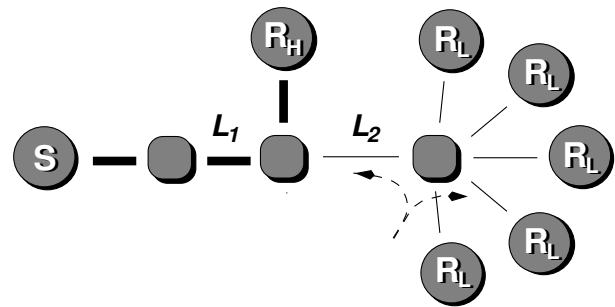
Figure 5: Shared Learning
