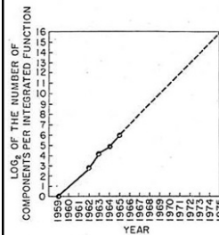
Fig. 2 Number of components per integrated function (at minimum cost per component extrapolated vs time).
