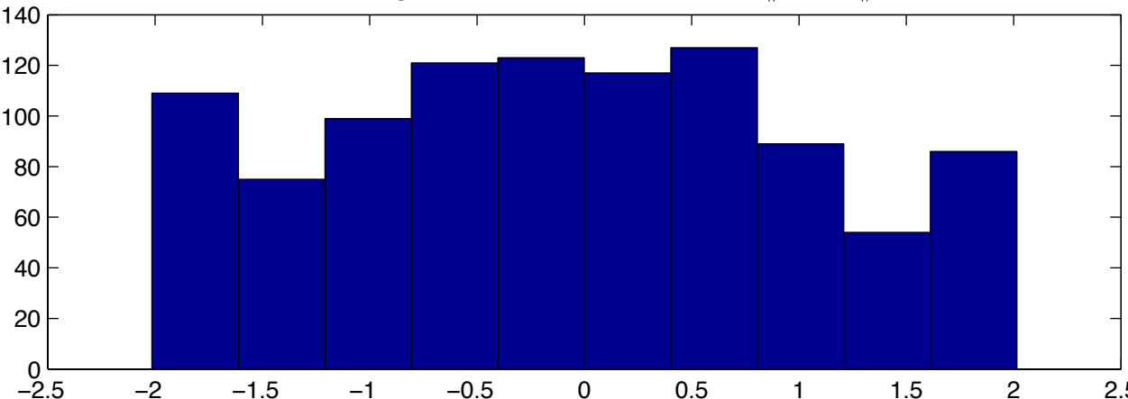
histogram of Ax - b at minimum of \|Ax - b\|_\infty
