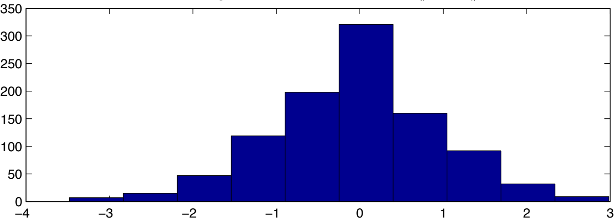
histogram of Ax - b at minimum of \|Ax - b\|_1
