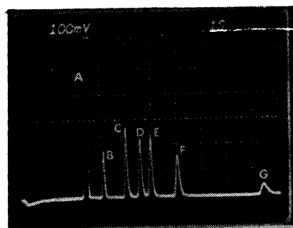
Fig. 27. Example of an output from the miniature gas chromatograph shown in Fig. 26. A) nitrogen; B) pentane; C) dichloromethane; D) chloroform; E) 11 l-trichloroethane; F) trichloroethylene; G) toluene. Photo courtesy of J. Jerman and S. Terry.
