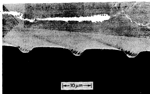
Fig. 9. SEM profile of laser-etched grooves [56]. The horizontal bar indicates 10 \text{ }\mu\text{m} . Conditions were 100 torr \text{Cl}_2 , 5.5-W multiline argon-ion laser, f/10 focusing, single scan at 90 \text{ }\mu\text{m}/\text{s} . Photo courtesy of D. Ehrlich.
