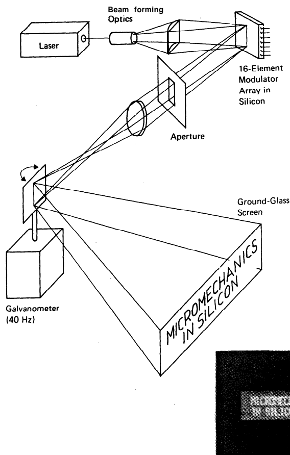
Fig. 49. Schematic of simple optical display employing the 16-beam array in Fig. 47. Each beam is operated as a single modulating element for the corresponding horizontal fine in the display. The inset shows a photograph of the display projected onto the ground glass screen.
