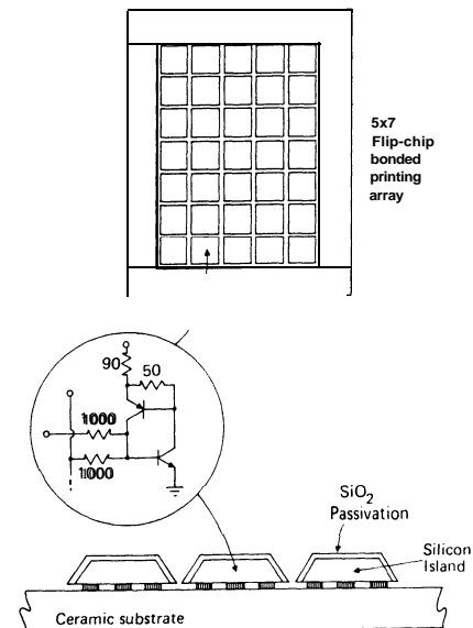
Fig. 63. A 5 \times 7 array of silicon islands forms the complete print head in the T.I. Silent 700 computer terminals. Each island is about 25\text{ }\mu\text{m} thick and contains the bipolar power latching circuit shown, yet this thin silicon IC chip is also forcefully abraded against the paper while simultaneously thermally cycled to 260^\circ\text{C} . Adapted from [174].
