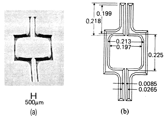
Fig. 41. (a) SEM of typical torsion mirror (tilted 60^\circ ) and (b) measured dimensions of 15-kHz mirror element (in cm). The SEM photo is a view of the mirror from the back surface where the electrostatic fields are applied.
