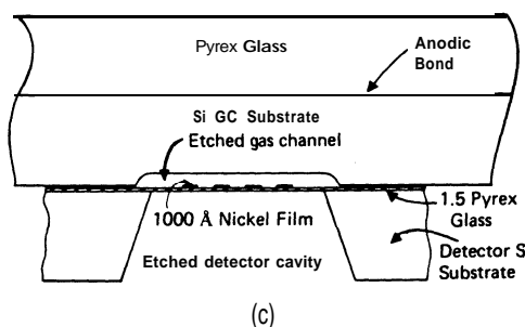
Fig. 26. The most ambitious project utilizing the mechanical properties of silicon is the Stanford gas chromatograph [29], [103]. (a) Overall view of the full silicon wafer showing 1) sample input, 2) purge input, 3) valve region, 4) exhaust of unused sample, 5) sensor region, 6) separation column. The various etched grooves are sealed by anodically bonding a glass plate over the entire wafer. A cross section of the valve assembly is drawn in (b) including the valve cavity, seating ring, and input orifice etched into the silicon as well as the thin nickel diaphragm. The thin-film thermal detector in (c) is also silicon based, consisting of a metal resistor evaporated on \text{SiO}_2 , thermally isolated by etching the silicon from beneath. Figures courtesy of J. Jerman and S. Terry.
