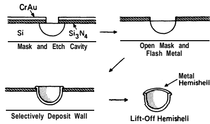
Fig. 14. Fabrication sequence for free-standing metal hemisells using an isotropic silicon-etching technique [78]. Typical dimensions of the hemisell are 350- \mu\text{m} diameter with a 4- \mu\text{m} -thick wall. Courtesy of K. D. Wise.
